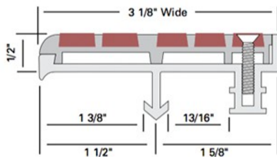
TYPE WP-RN3SG 3 1/8" (79.375 mm) wide 1/2" (12.7 mm) thick
