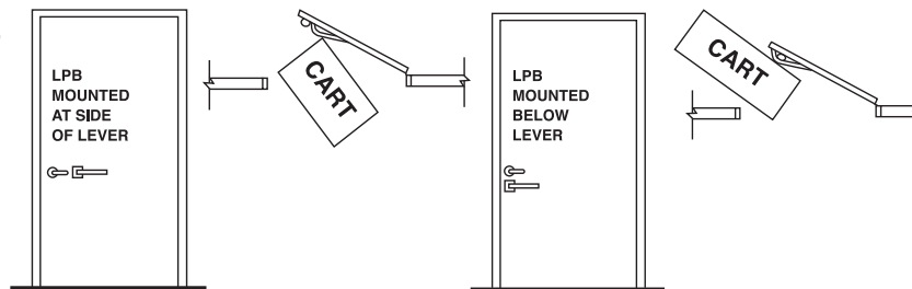
Application shown for product R101LPB thru R115LPB. * Advise if door thickness is other than 1 3 / 4 ".
