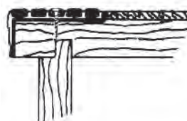
Type 142 Supergrit® attached to wood tread and backed with tile, carpet, or other material.
