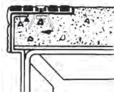
Type 133 Supergrit® with wing anchors in concrete filled steel pan.
