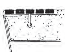
TYPE 231 BF Sure-Hold anchor in sloped riser steel pan step.
