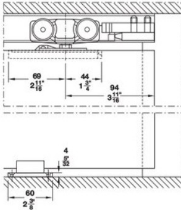
Section guide and trolley hanger
