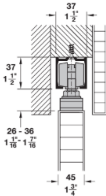
Ceiling installation with wood door
