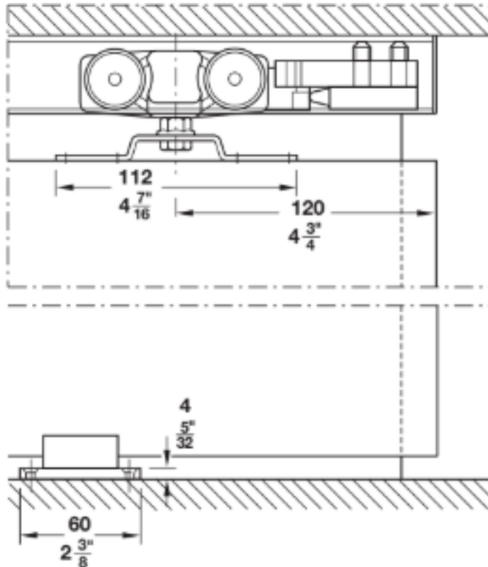
Section hanger and trolley guide
