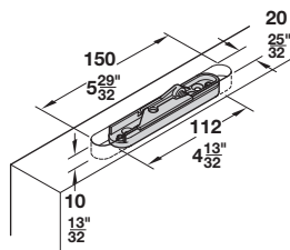
Routing dimensions for support flange
