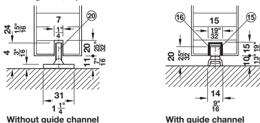
Without guide channel
