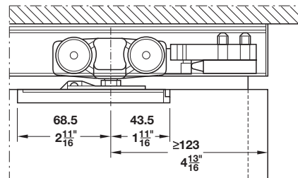
Classic 240-O section trolley hanger
