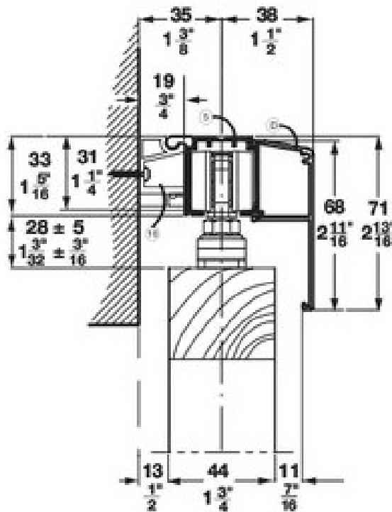
1 3/4" door with wall mounted track 5 , fascia D and mounting rail 16
