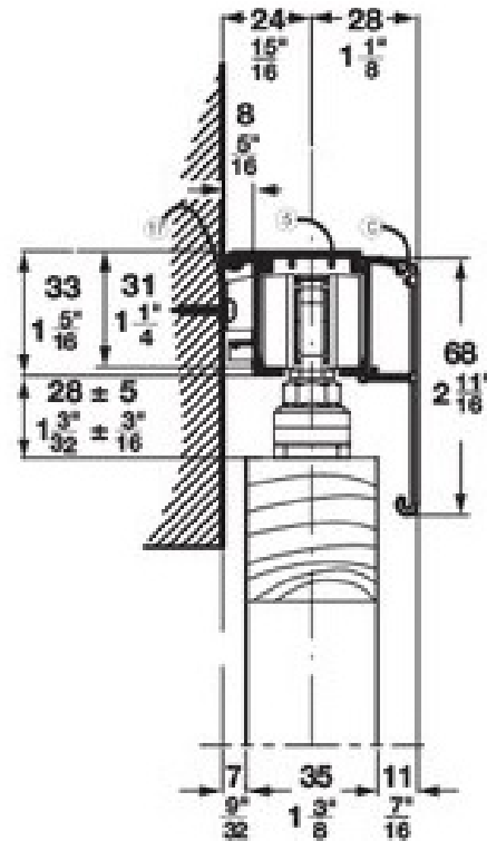
1 3/8" door with wall mounted track 5 , fascia clip C and mounting rail 17
