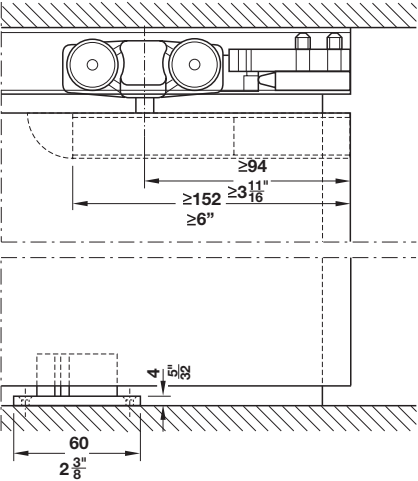
Section guide and trolley hanger
