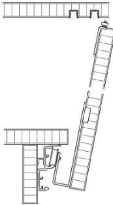
Mounting sliding door to cabinet
