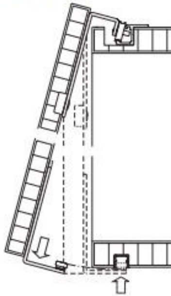
Mounting Sliding Door to Cabinet
