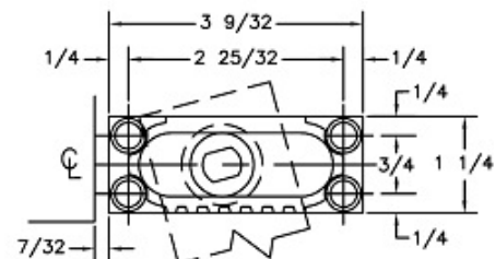
FLOOR GEAR BOX- PLAN VIEW
