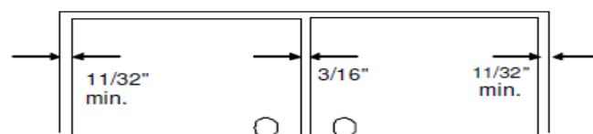
PAIR OF DOORS - SQUARE EDGED
