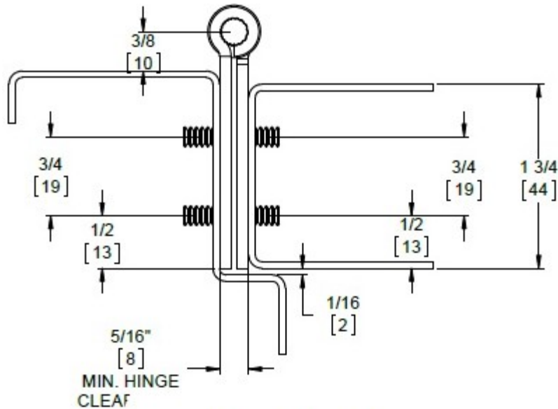
Door Closed
