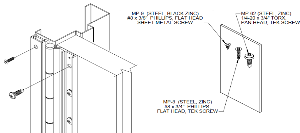
FIGURE 2: INSTALLATION (EXPLODED VIEW)
