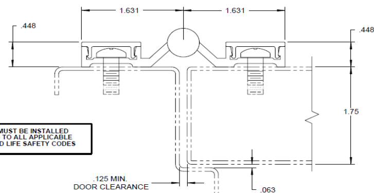
FIGURE 1: HINGE PLACEMENT & CLEARANCE TEMPLATE
