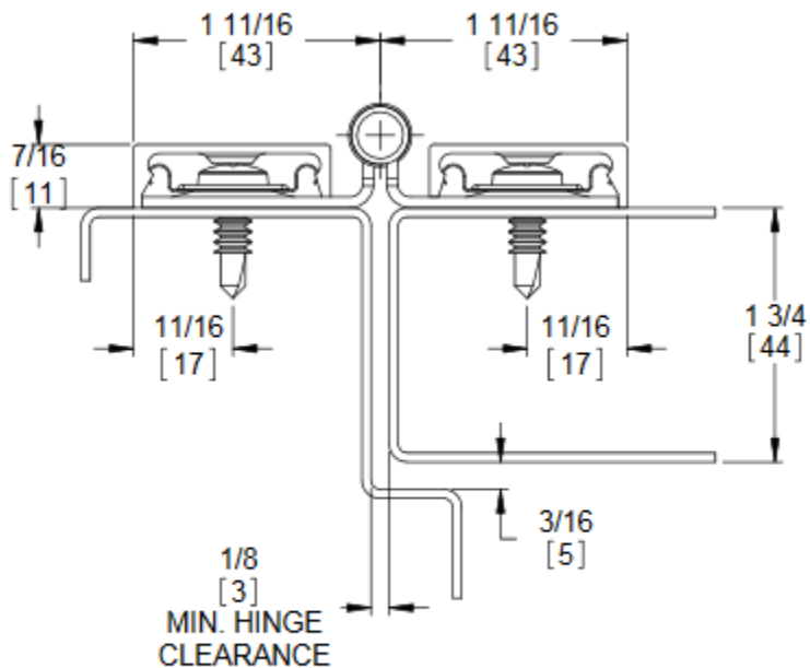
Door Closed
