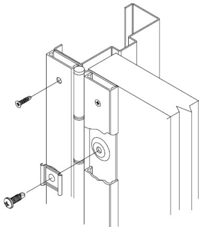
Figure 2: Installation (Exploded View)
