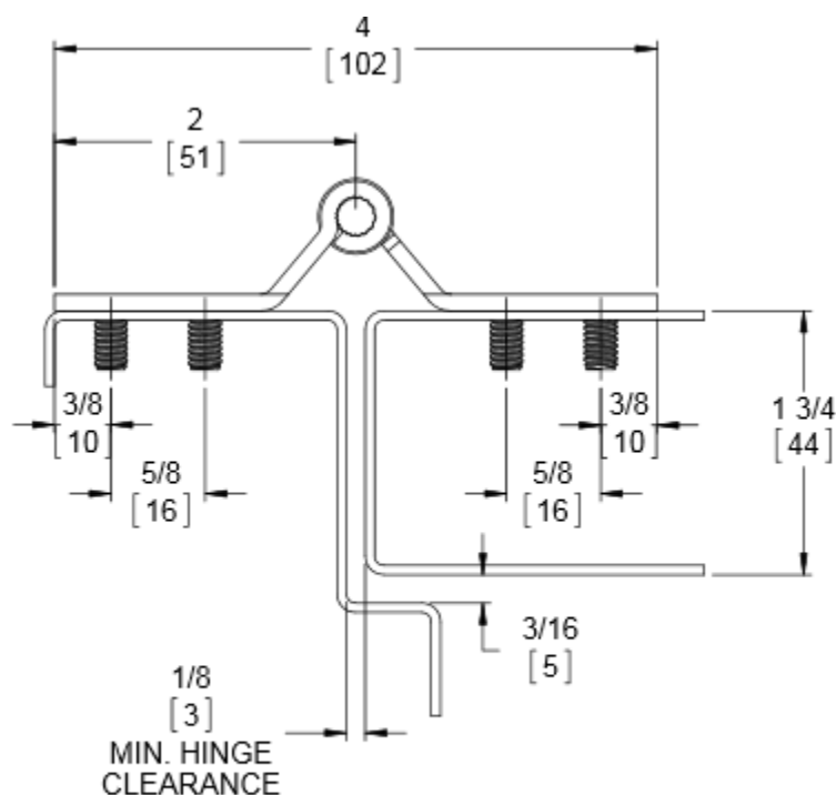
Door Closed
