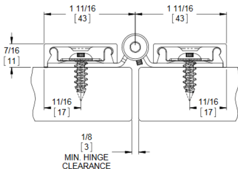
Door Closed
