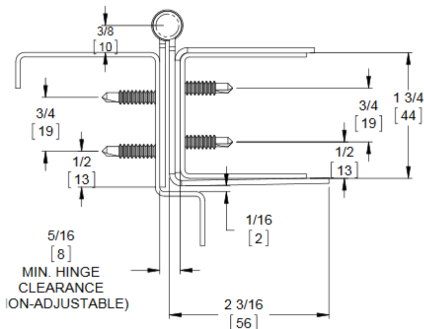
Door Closed
