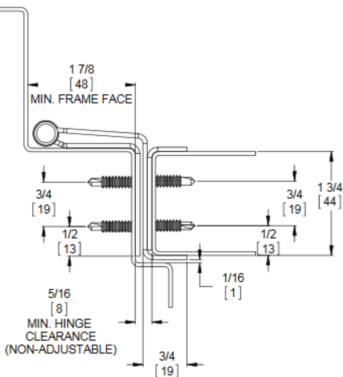
Door Closed
