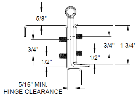
FIGURE 7: HINGE PLACEMENT & CLEARANCE TEMPLATE (NON- ADJUSTABLE APPLICATION SHOWN)
