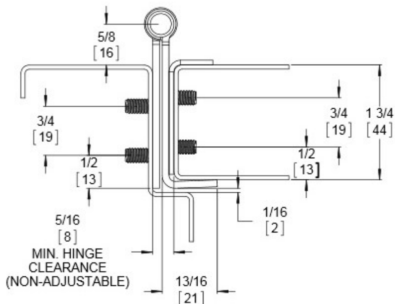
Door Closed
