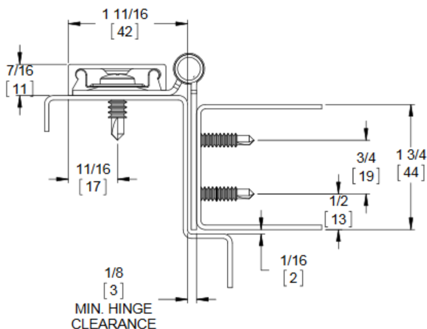
Door Closed
