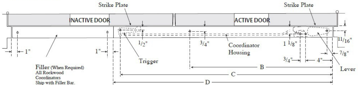
PLAN VIEW OF DOORS AND FRAME
