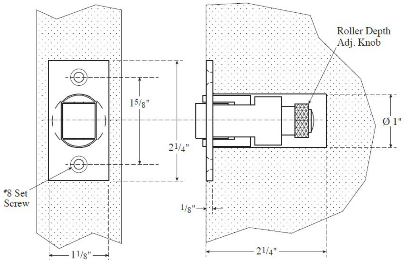
Strike Detail
