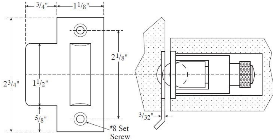
Strike Detail
