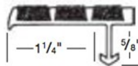
TYPE 121BF 1 7/8" (47.6 mm) wide 1/4" (6.35 mm) thick
